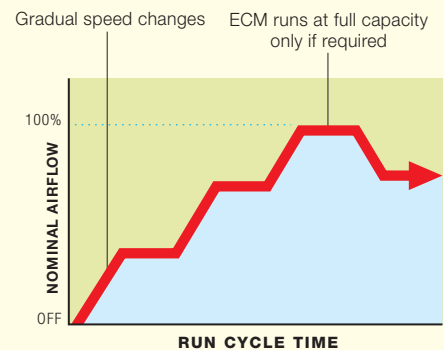
Extended run times at reduced speeds help to control humidity and reduce noise.
